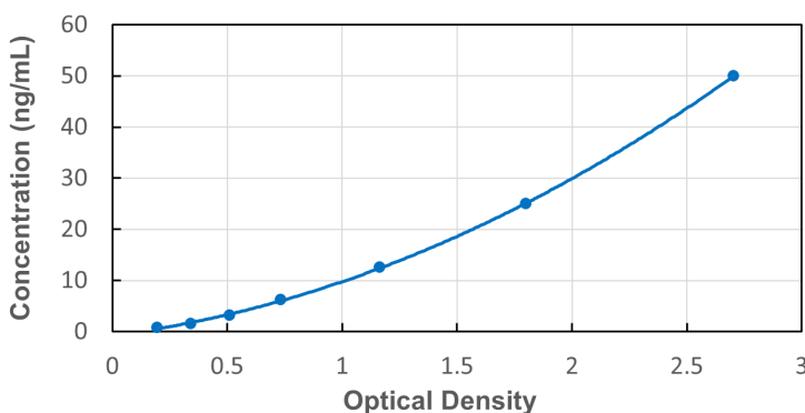
Typical Standard Curve for Human SEMA5A ELISA
