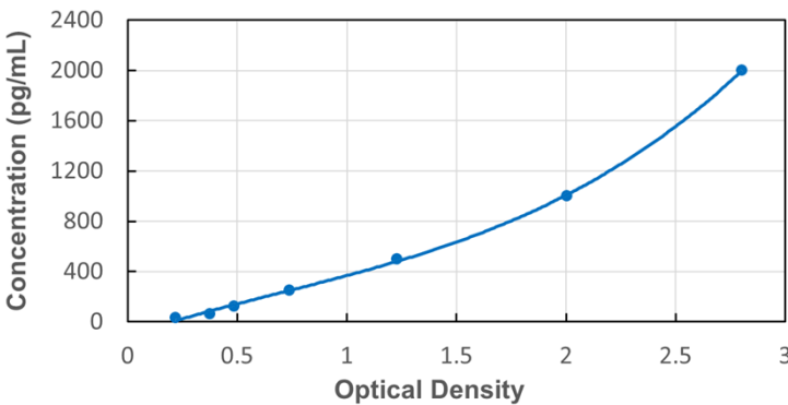
Typical Standard Curve for Human DUSP1 ELISA
