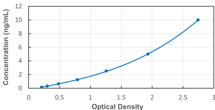
Typical Standard Curve for Mouse FXR ELISA
