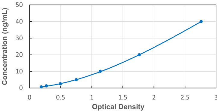
Typical Standard Curve for Human MAT1a ELISA
