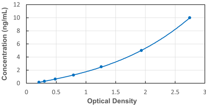
Typical Standard Curve for Human SNAP25 ELISA
