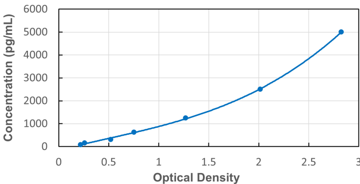
Typical Standard Curve for Human ABCA3 ELISA
