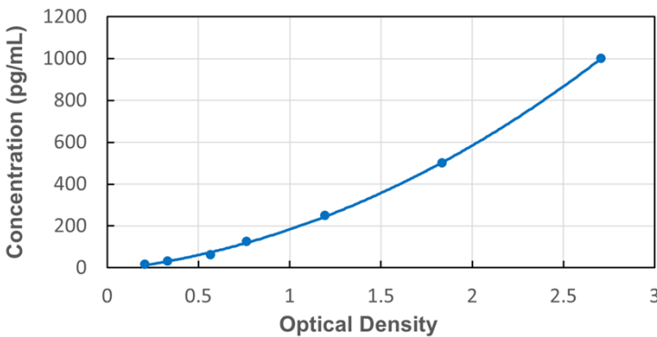
Typical Standard Curve for Human ADH2 ELISA
