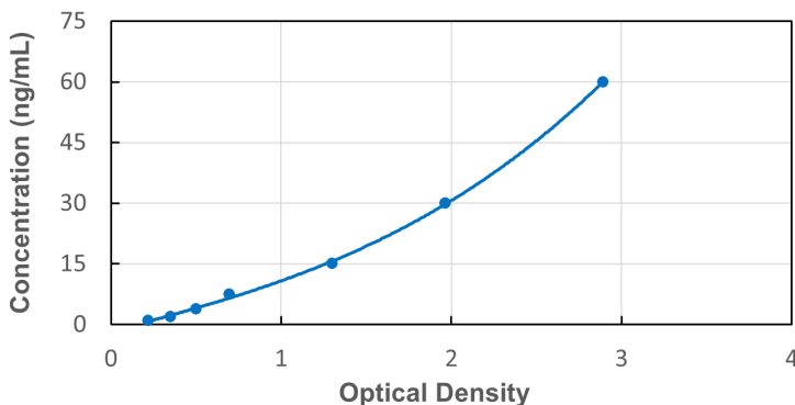
Typical Standard Curve for Mouse AT ELISA
