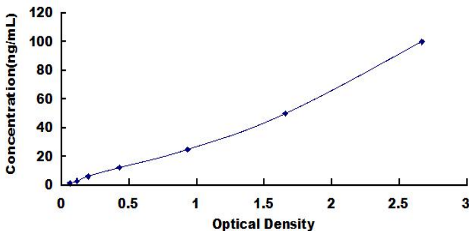
Typical Standard Curve for AGC ELISA.
