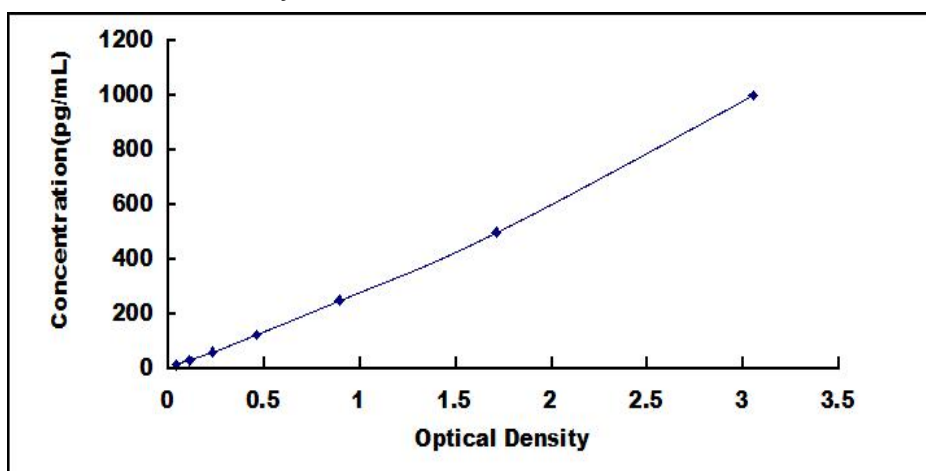
Typical Standard Curve for ALDOA ELISA.
