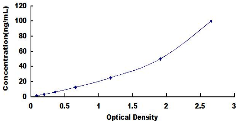
Typical Standard Curve for AHSG ELISA.
