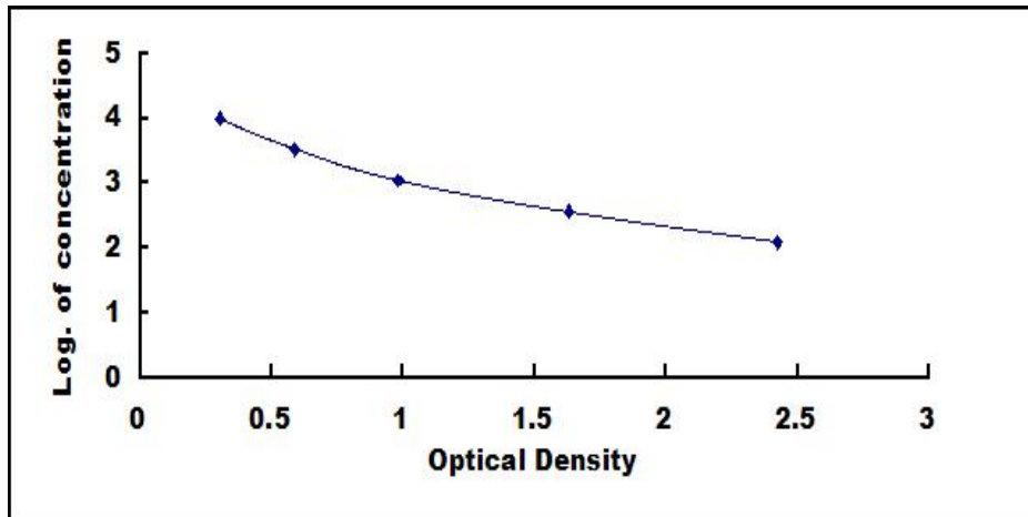
Typical Standard Curve for ASD ELISA.
