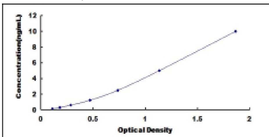
Typical Standard Curve for ATP4a ELISA.
