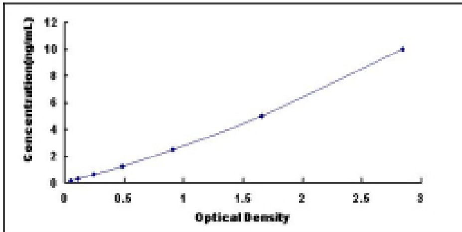
Typical Standard Curve for BHLHB8 ELISA.
