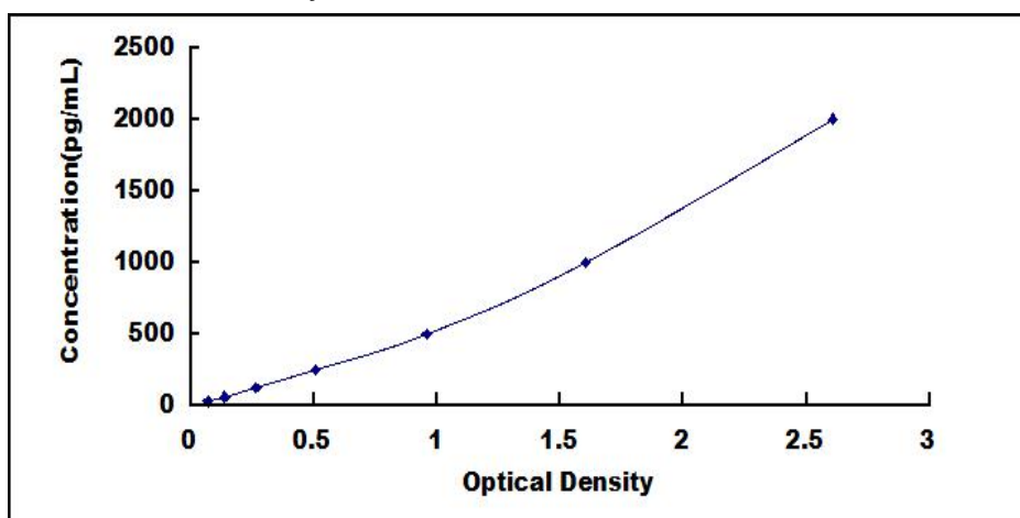
Typical Standard Curve for BMP3 ELISA.
