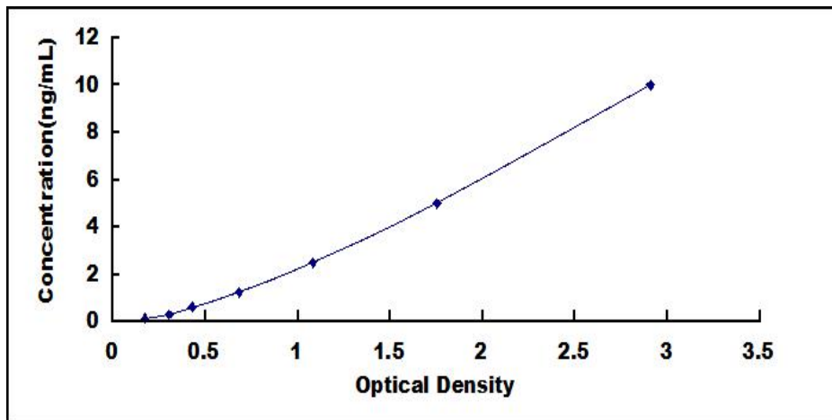
Typical Standard Curve for CA5B ELISA.
