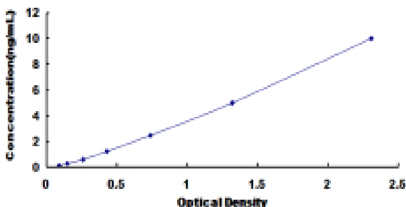
Typical Standard Curve for CTSG ELISA.
