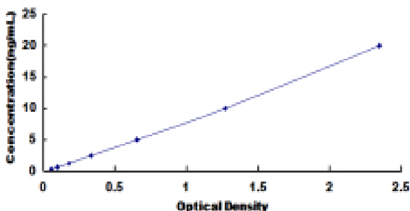
Typical Standard Curve for CAT1 ELISA.
