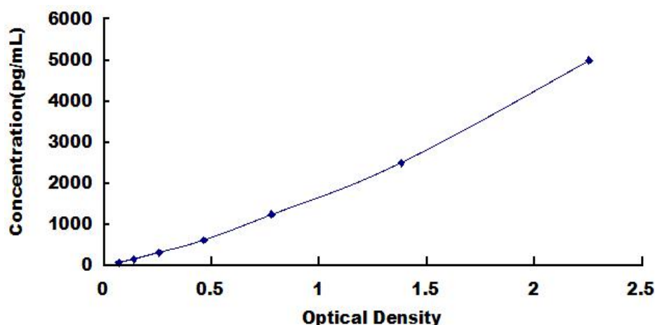
Typical Standard Curve for CAV1 ELISA.
