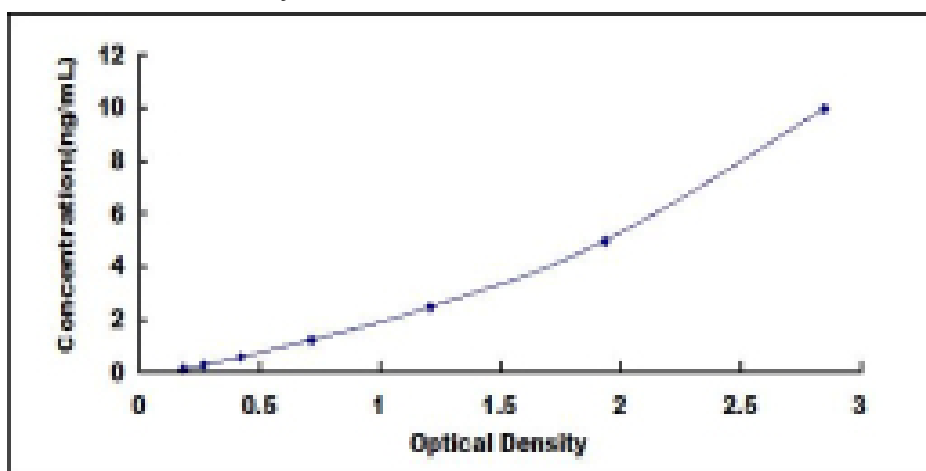
Typical Standard Curve for CLC ELISA.
