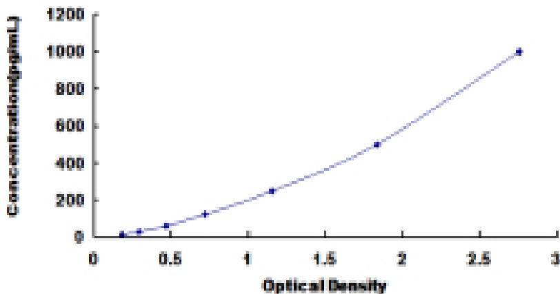
Typical Standard Curve for GCSF ELISA.
