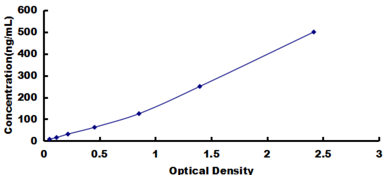
Typical Standard Curve for C4d, Human ELISA.
