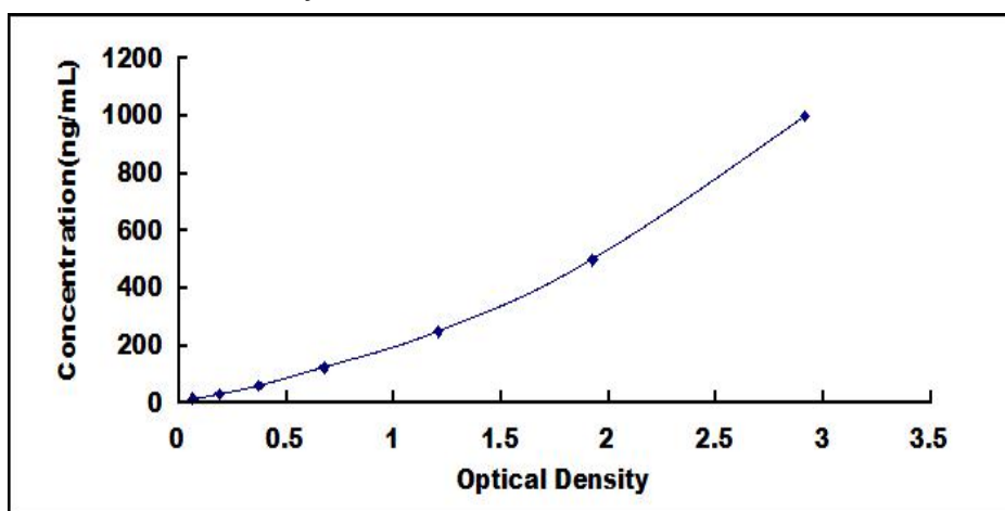
Typical Standard Curve for CFP ELISA.
