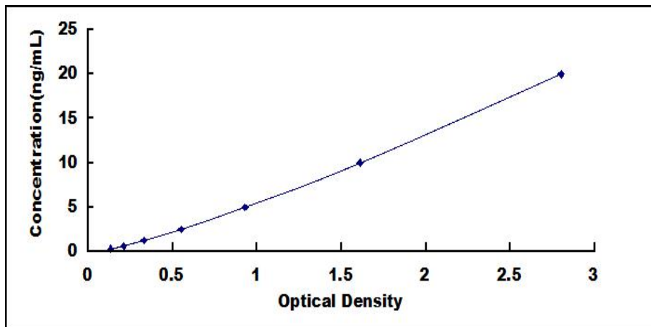
Typical Standard Curve for CRT ELISA.
