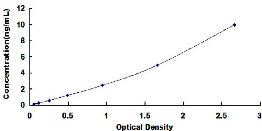
Typical Standard Curve for CRKL ELISA.
