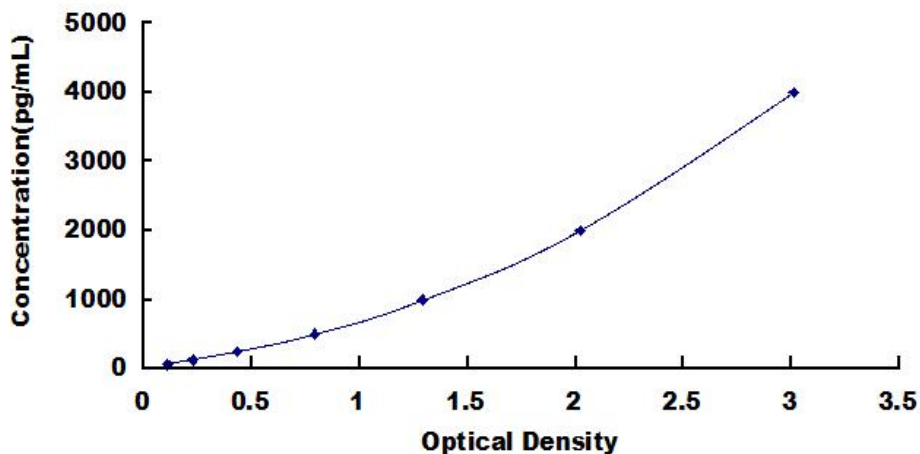
Typical Standard Curve for CNP ELISA.
