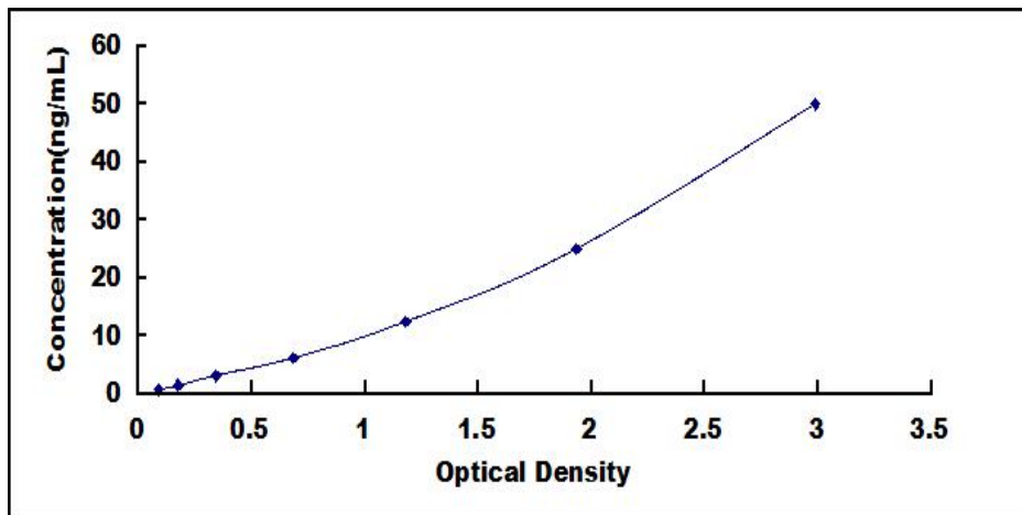
Typical Standard Curve for CDA ELISA.
