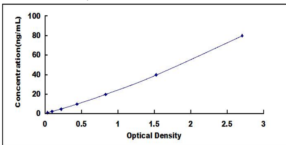
Typical Standard Curve for DCN ELISA.
