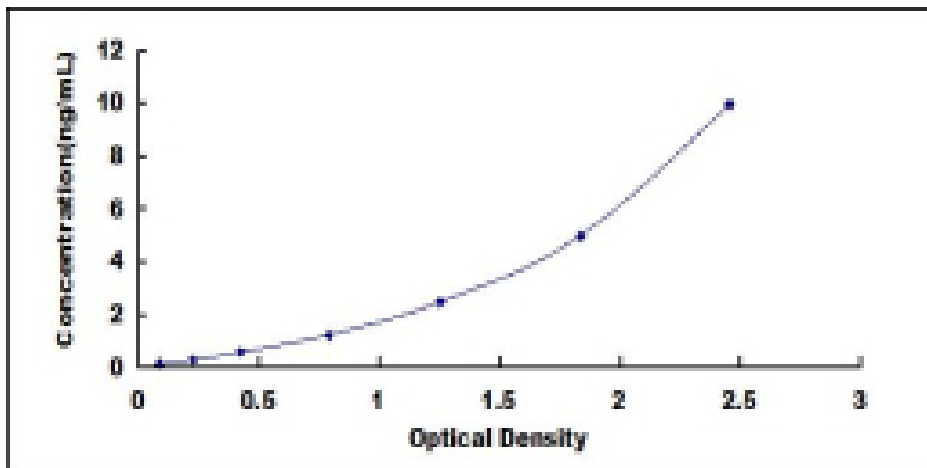
Typical Standard Curve for DCK ELISA.
