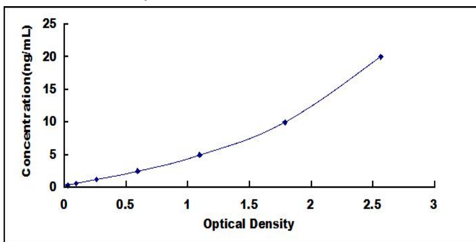
Typical Standard Curve for DSE ELISA.
