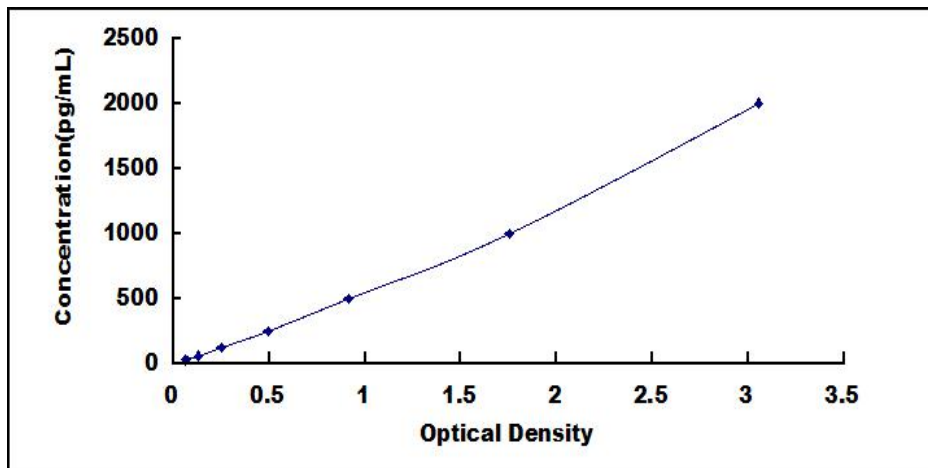
Typical Standard Curve for ECE1 ELISA.
