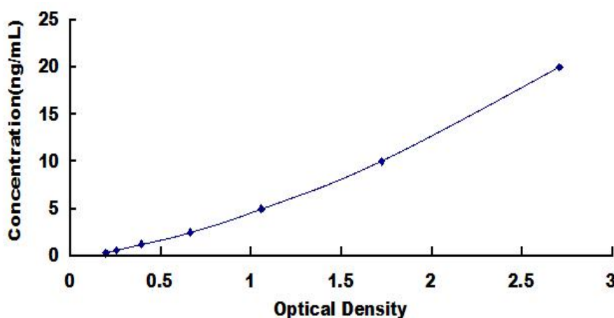
Typical Standard Curve for EGFR ELISA.
