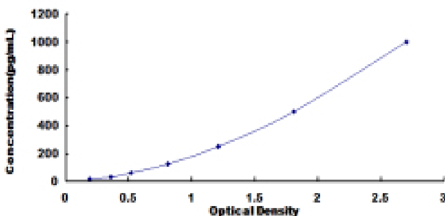
Typical Standard Curve for ENA78 ELISA.
