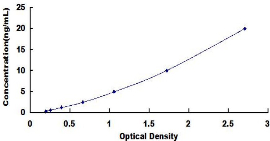
Typical Standard Curve for ERb ELISA.
