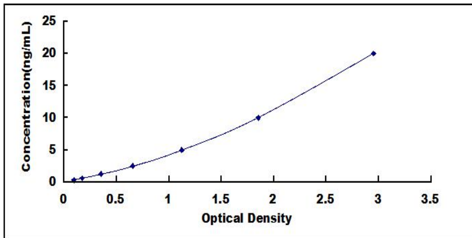
Typical Standard Curve for GRa ELISA.
