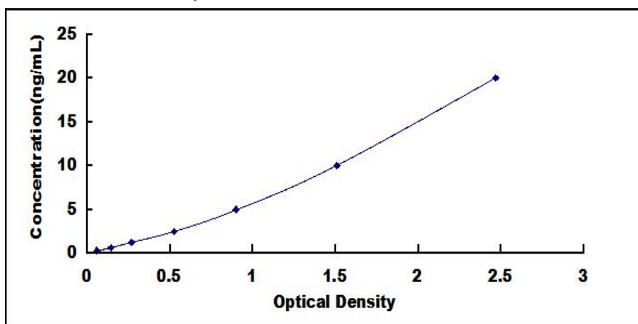
Typical Standard Curve for GLS ELISA.
