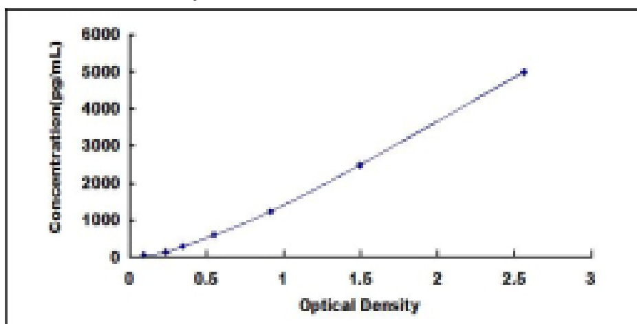
Typical Standard Curve for GR ELISA.
