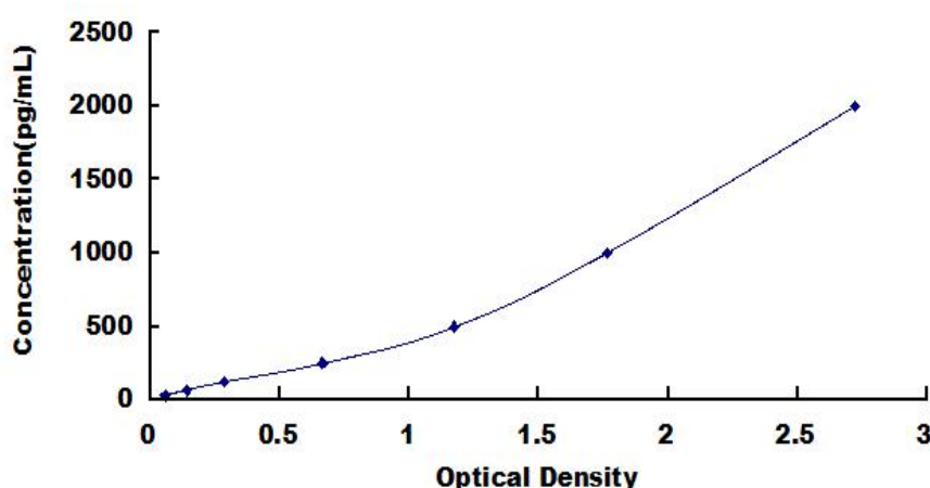
Typical Standard Curve for GRN ELISA.
