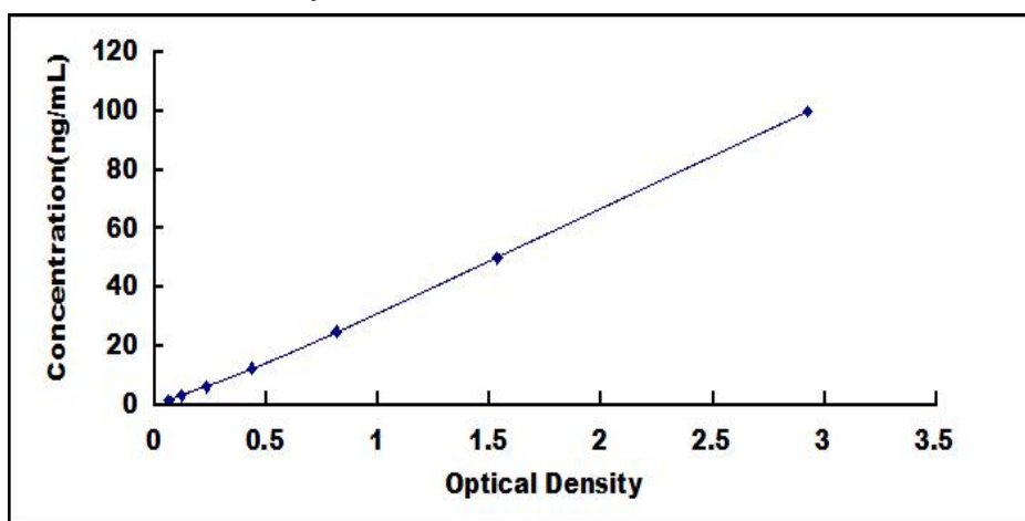
Typical Standard Curve for HSP10 ELISA.
