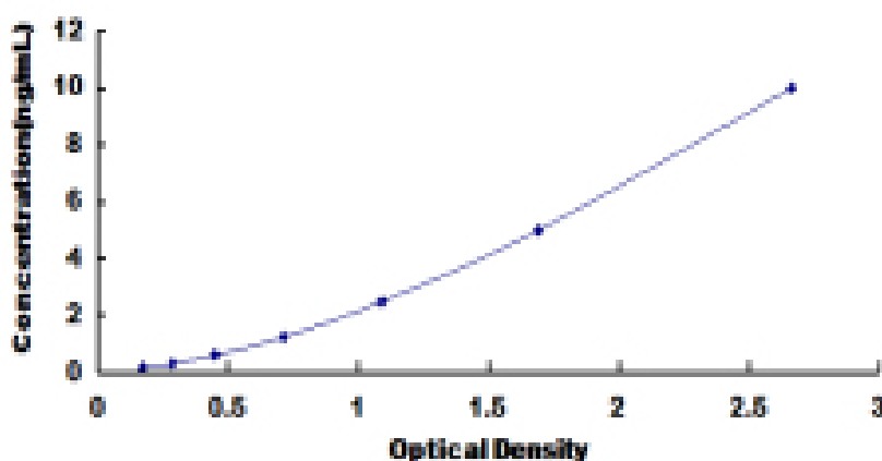
Typical Standard Curve for HRH4 ELISA.
