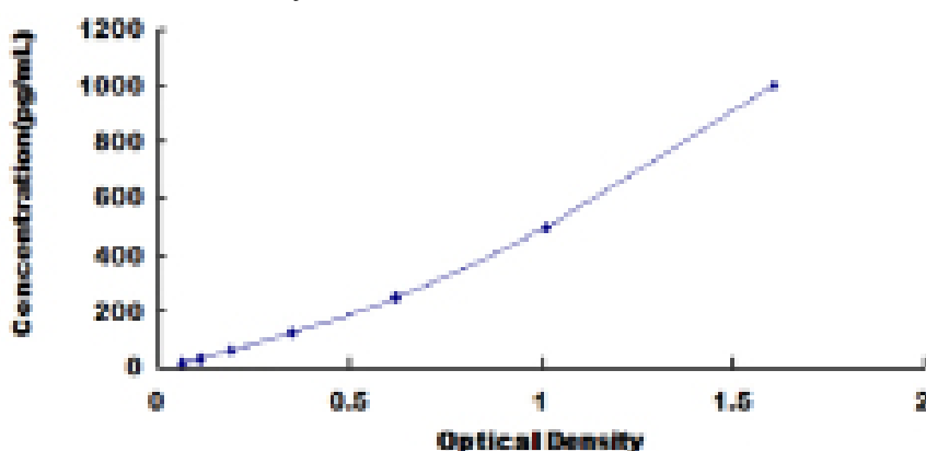
Typical Standard Curve for IL3, Canine ELISA.
