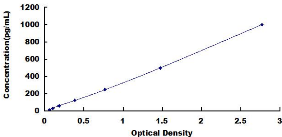
Typical Standard Curve for IL7 ELISA.
