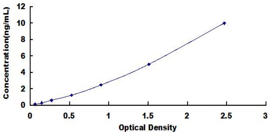
Typical Standard Curve for LDH ELISA.
