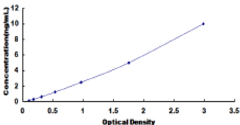
Typical Standard Curve for LDLRAP1 ELISA.
