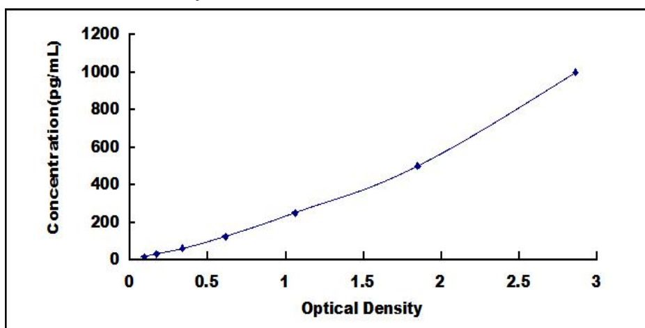
Typical Standard Curve for MPI ELISA.
