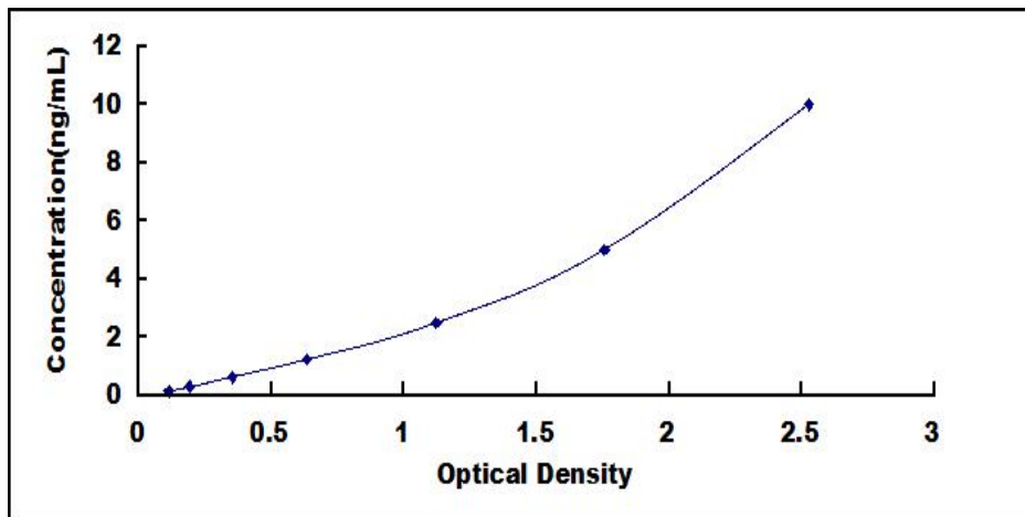
Typical Standard Curve for MMP25 ELISA.
