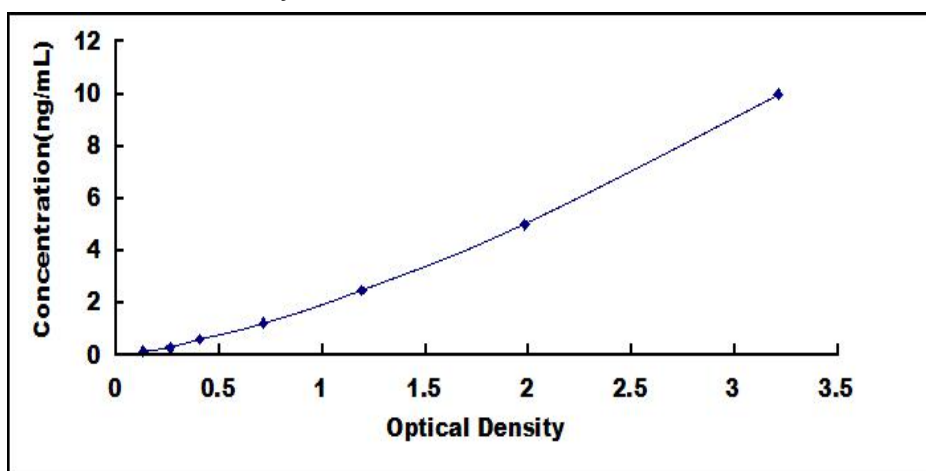
Typical Standard Curve for MK ELISA.
