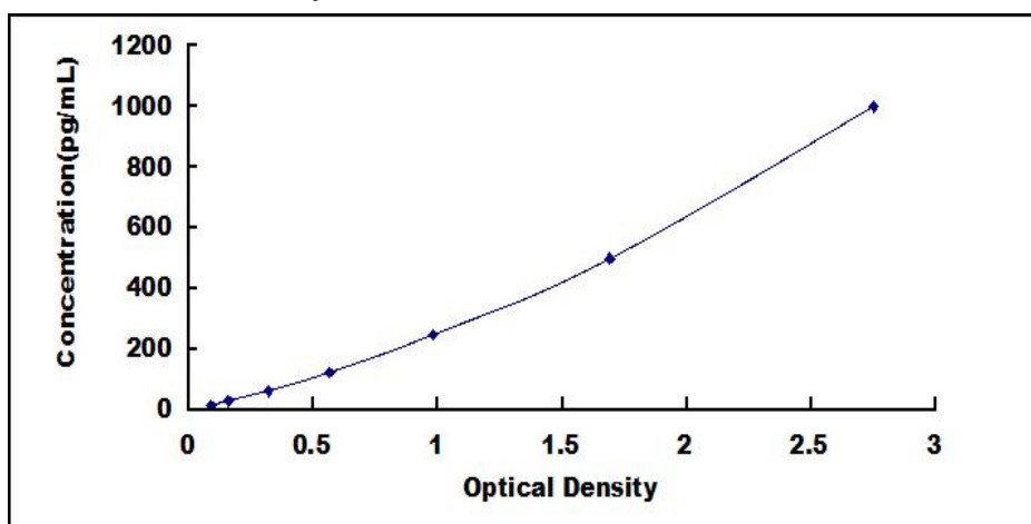
Typical Standard Curve for PLUNC ELISA.
