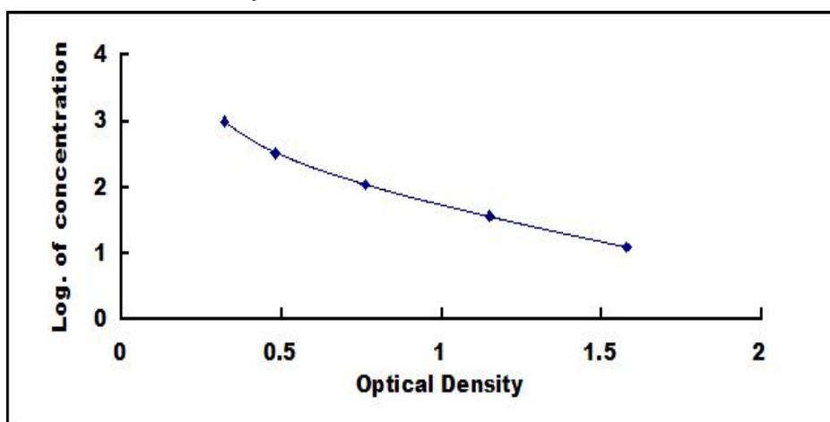
Typical Standard Curve for PYY3 ELISA.
