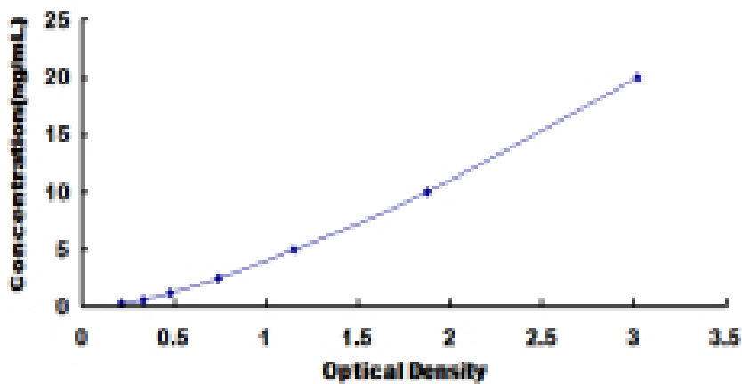
Typical Standard Curve for PLIN4 ELISA.
